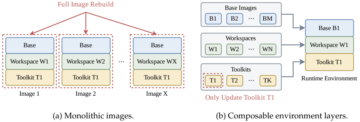
Figure 4 | Impact of upgrading Toolkit T1 under two environment packaging schemes. (a) With monolithic images, every image embedding T1 must be rebuilt even though its base image and workspace are unchanged. (b) With independently versioned composable layers, only the T1 layer is updated and then recombined with existing base-image and workspace layers.
